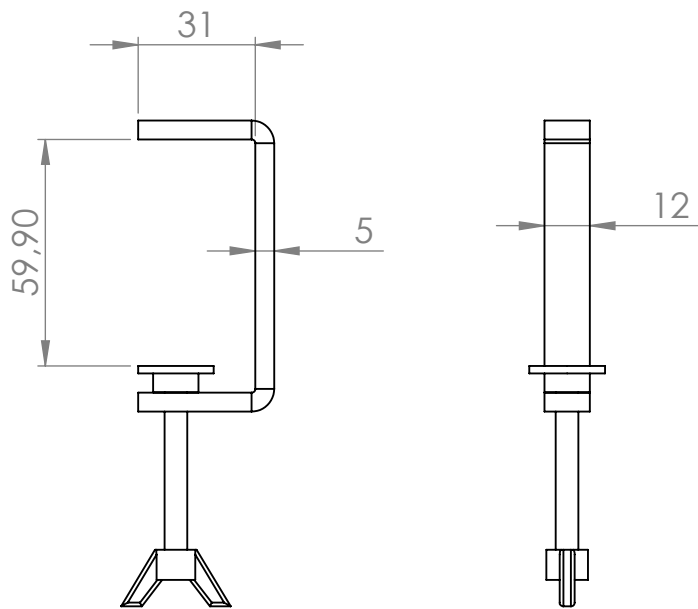
Clamp 2 pcs
